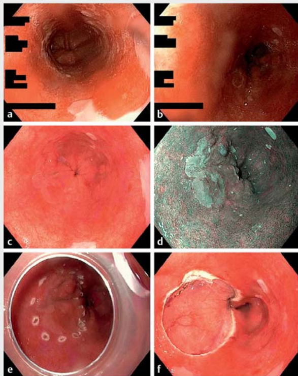
Fig. 2 Endoscopic images of a patient referred with confirmed low grade dysplasia (LGD) in random biopsies; no visible lesions were detected at the referring hospital. Images from the community hospital ( a, b ) and the Barrett Expert Center (BEC) ( c–f ). a, b Images in white-light endoscopy (WLE) of a C4M5 Barrett's segment without signs of reflux esophagitis. The endoscopist reported no visible abnormalities and took random biopsies at three levels (i. e. unclear whether these were taken by following the Seattle protocol). Histopathology analysis showed LGD in all three levels, with p53 expression. Panel review confirmed the diagnosis. c, d Images in WLE and narrow-band imaging of the same patient with a Barrett's segment containing a Paris type 0-IIa visible lesion of 25 mm in diameter, 2 cm above the gastroesophageal junction, at the 7–11 o'clock neutral position. e Endoscopic view through the Duette cap: lesion delineated with electrocoagulation markers before starting the endoscopic resection procedure. f View of the wound after resection and removal of the cap. Histopathology analysis showed esophageal adenocarcinoma invading the submucosa, with good differentiation, without signs of lymphovascular invasion.
